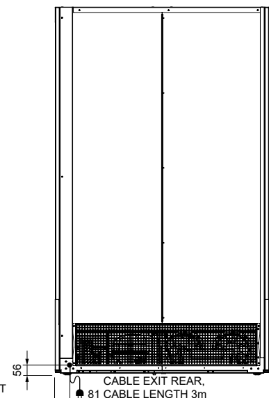
REAR ELEVATION
