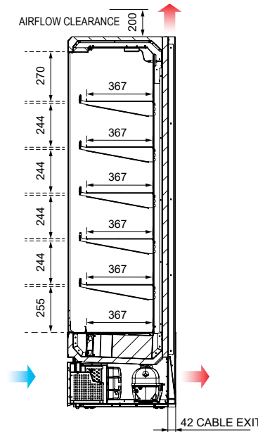
SECTION VIEW
