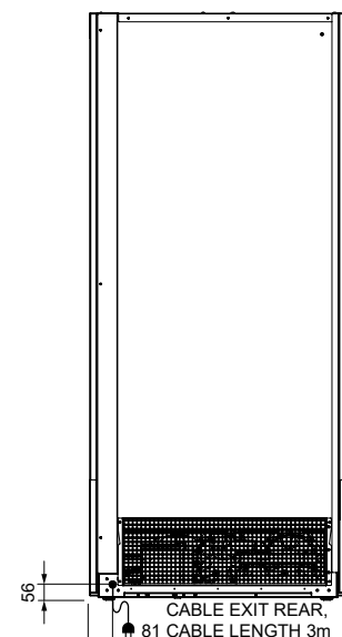
REAR ELEVATION
