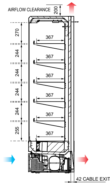
SECTION VIEW
