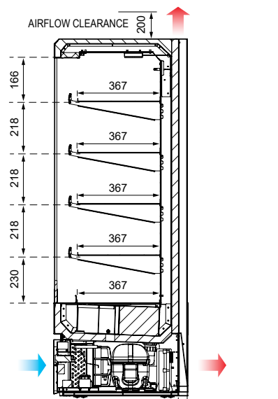
SECTION VIEW
