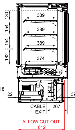
SECTION VIEW
