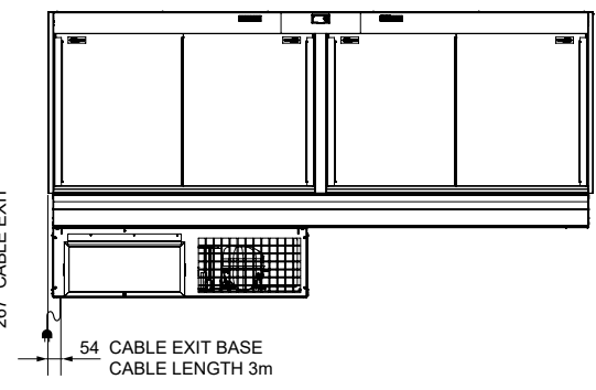
REAR ELEVATION
