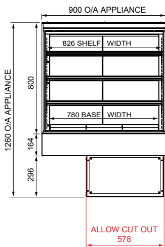
FRONT ELEVATION
