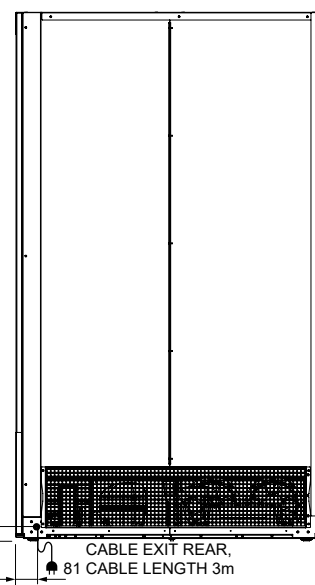
REAR ELEVATION
