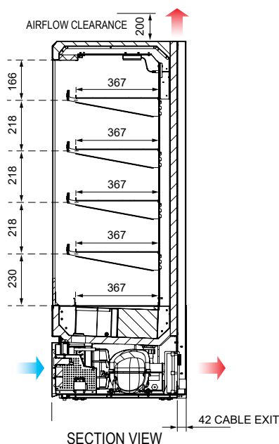
SECTION VIEW
