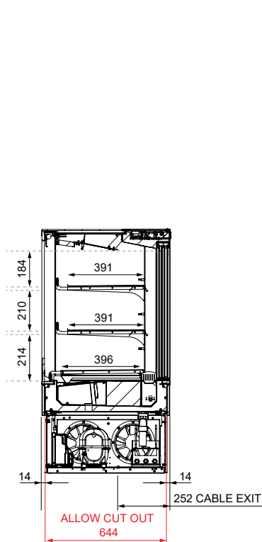
SECTION VIEW
