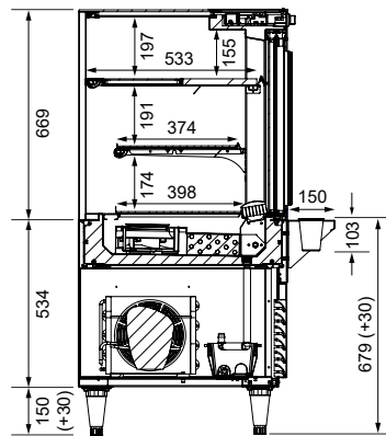
SECTION VIEW
