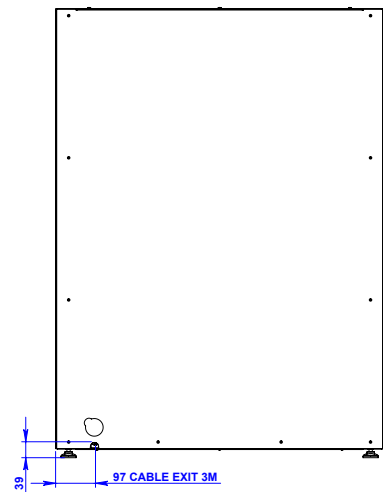
REAR ELEVATION
