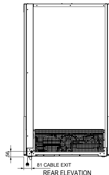
REAR ELEVATION
