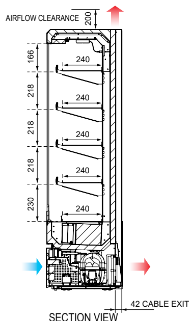
SECTION VIEW
