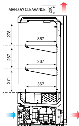
SECTION VIEW
