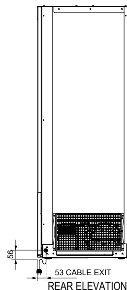
REAR ELEVATION
