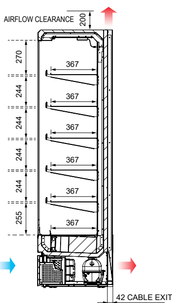
SECTION VIEW
