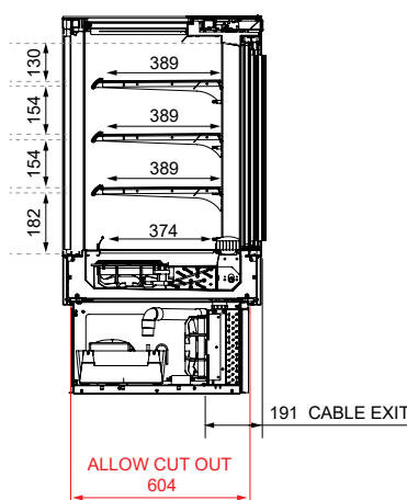
SECTION VIEW
