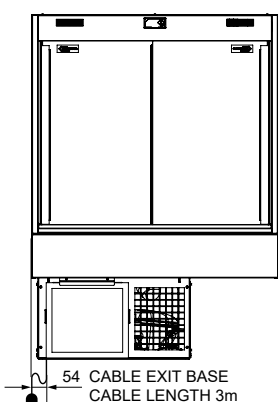
REAR ELEVATION
