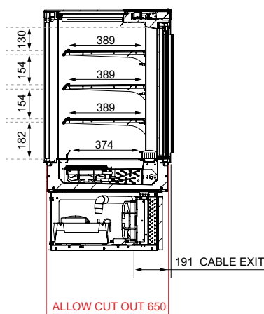
SECTION VIEW
