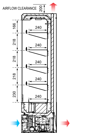
SECTION VIEW
