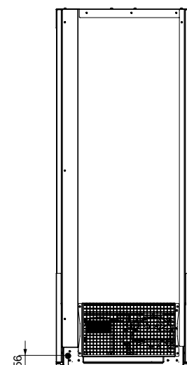
REAR ELEVATION
