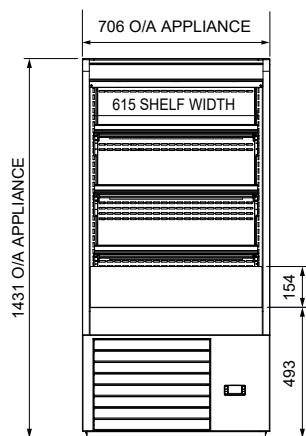
FRONT ELEVATION
