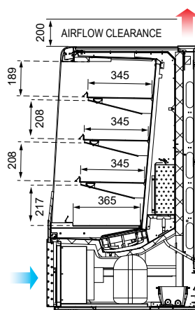
SECTION VIEW
