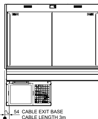
REAR ELEVATION
