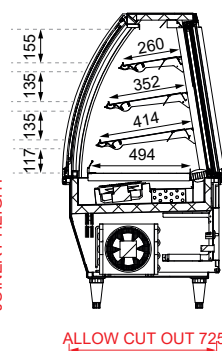
SECTION VIEW
