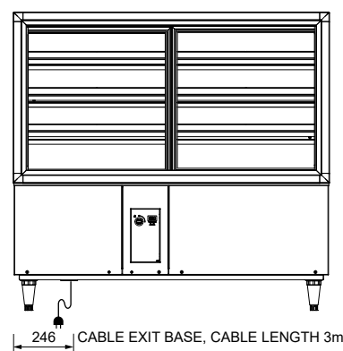
REAR ELEVATION
