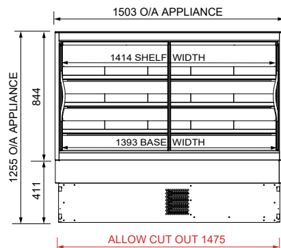
FRONT ELEVATION
