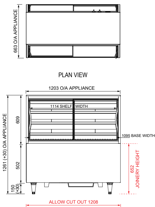
FRONT ELEVATION
