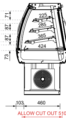
SECTION VIEW
