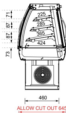
SECTION VIEW
