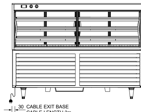
REAR ELEVATION
