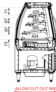
SECTION VIEW
