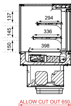
SECTION VIEW
