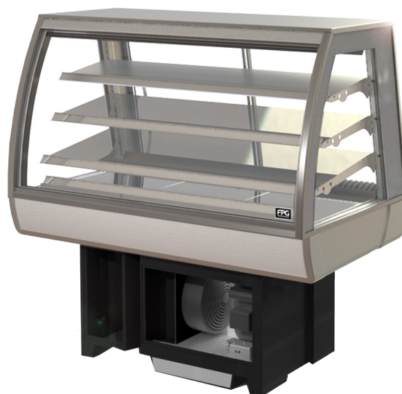
Showing : Inline 3000 Series refrigerated 1200mm curved on-counter fixed front with integral refrigeration
