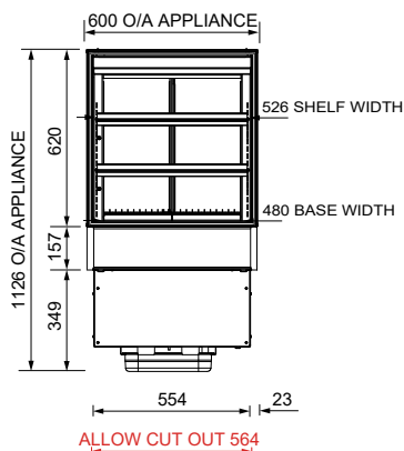
FRONT ELEVATION
