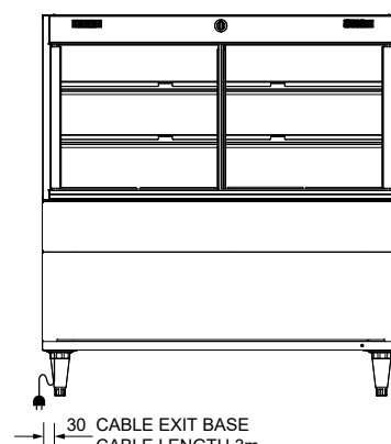
REAR ELEVATION
