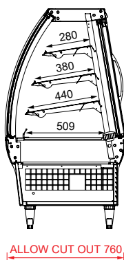
SECTION VIEW
