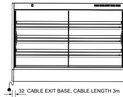
REAR ELEVATION
