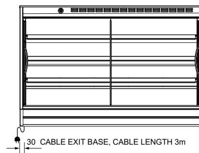
REAR ELEVATION
