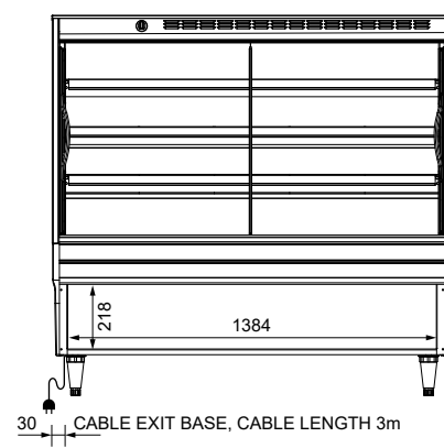
REAR ELEVATION
