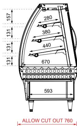
SECTION VIEW
