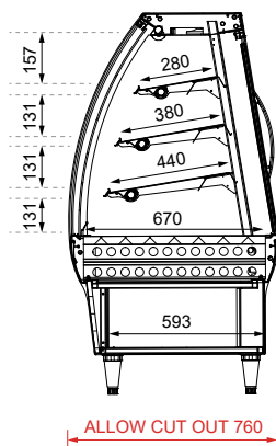
SECTION VIEW
