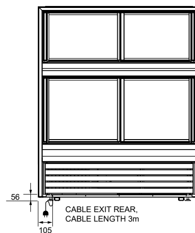
REAR ELEVATION
