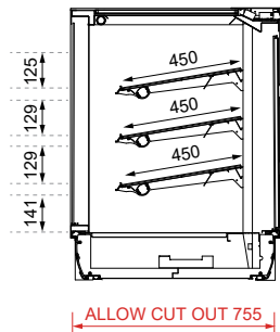
SECTION VIEW
