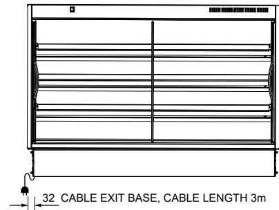
REAR ELEVATION
