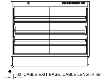
REAR ELEVATION
