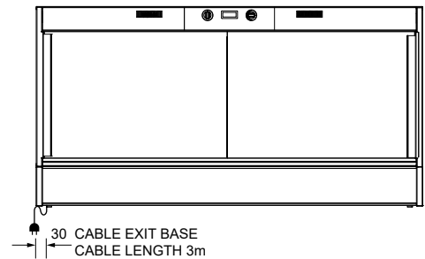
REAR ELEVATION
