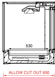
SECTION VIEW
