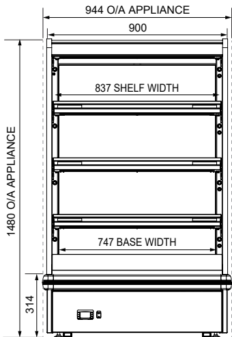
FRONT ELEVATION
