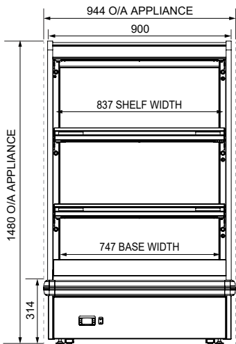
FRONT ELEVATION
