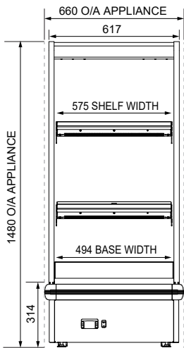
FRONT ELEVATION
