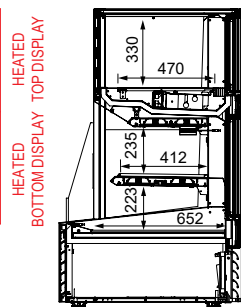
SECTION VIEW
