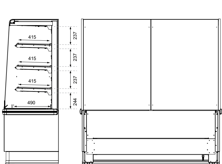
SECTION VIEW
