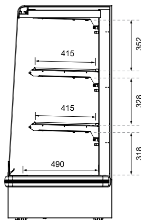
SECTION VIEW
