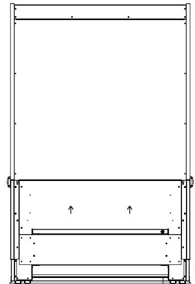
CABLE EXIT REAR, CABLE LENGTH 3m REAR ELEVATION
