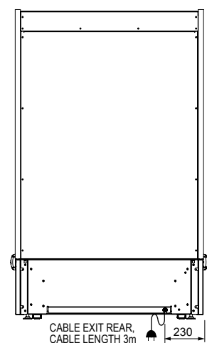
REAR ELEVATION
